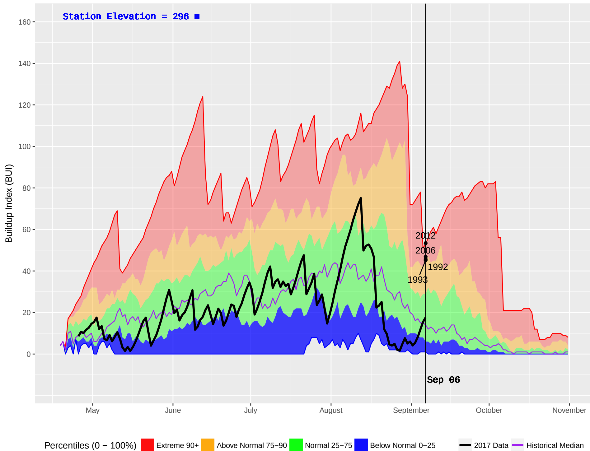
VAN DYKE (430) : Historical (1983–2016) and Current (2017) Noon Buildup Index (BUI)
