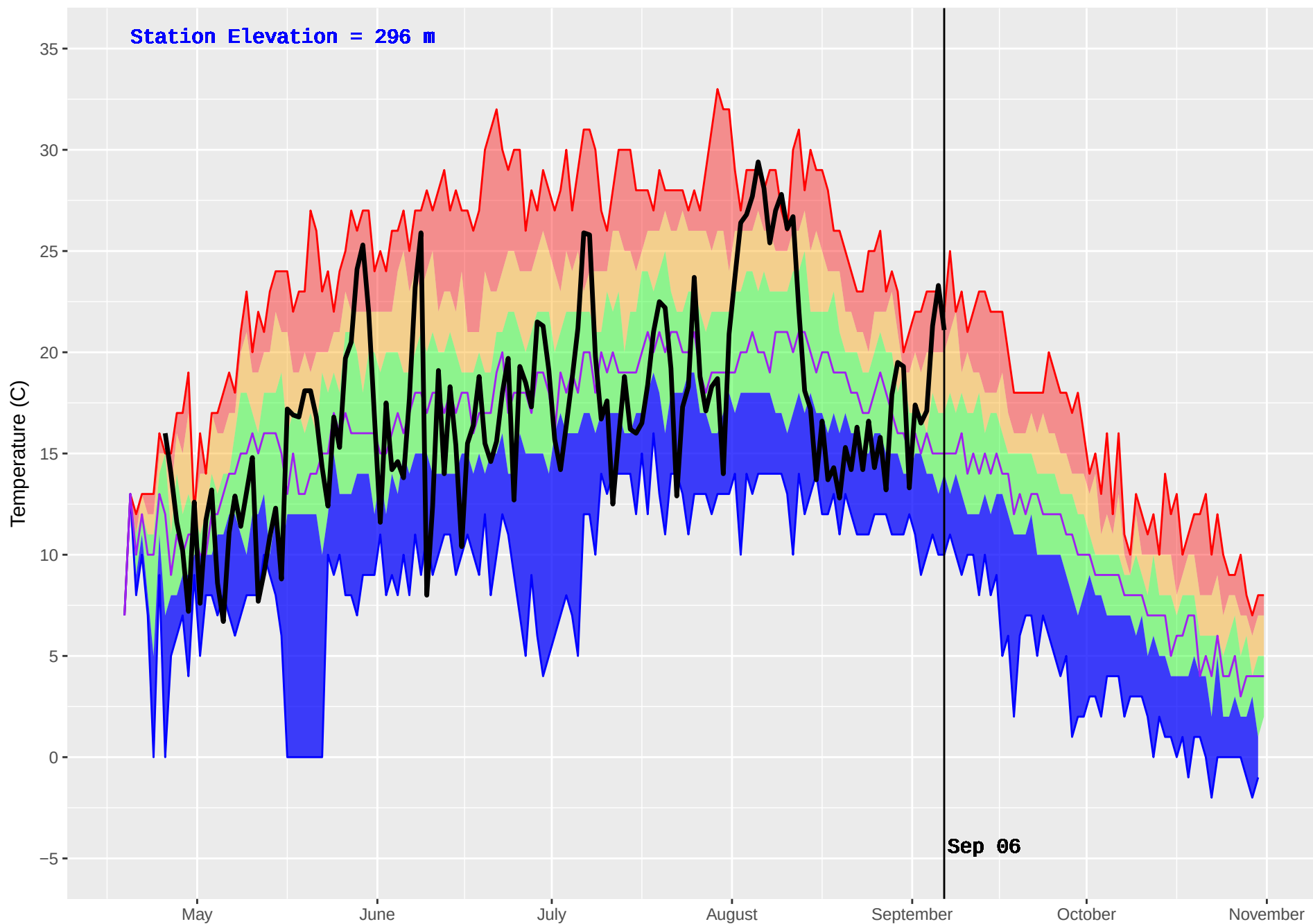
VAN DYKE (430) : Historical (1983–2016) and Current (2017) Noon Temperature
